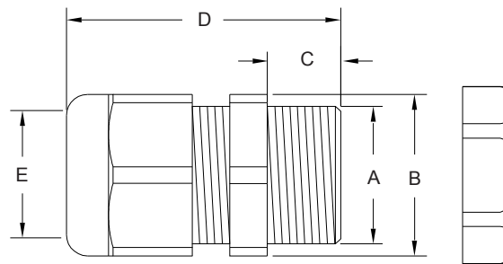
CanTop Strain Relief Connector
